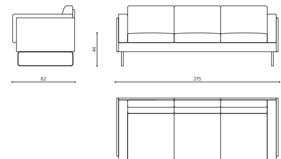
CA 3000 divano 3 posti • 3 seater sofa
